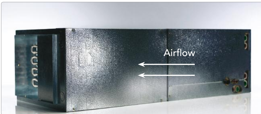
Flexible configurations: Upflow, Downflow and Horizontal
