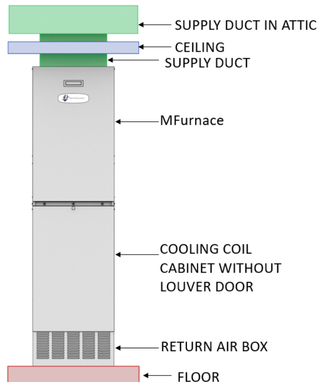
Figure 10: Typical upflow installation with supply duct and return air box
