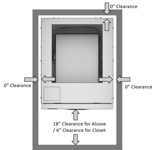
Figure 1: Clearance to service and combustibles
