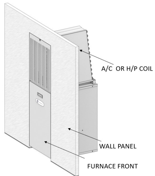
Figure 3: Example of Alcove installation
