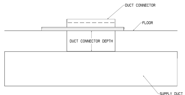
Figure 8: Duct connector location
