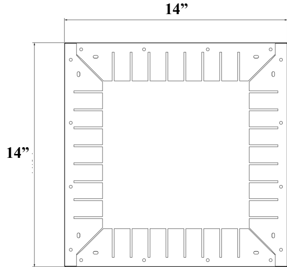
Figure 6: Duct connector dimension
