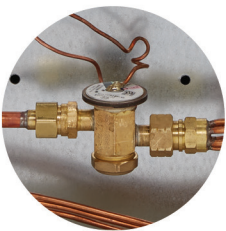
Factory installed TXV's with bolt on connections
